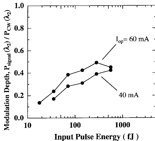
Fig. 4. Modulation depth (ratio of the output pulse intensity to the 1560-nm intensity inside the calcite) as a function of input pulse energy. The saturation originates from pulse-gain saturation in the SOA.
