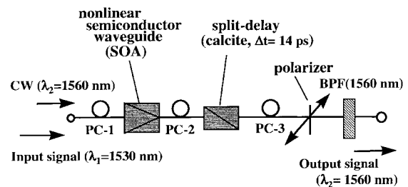
Fig. 1. Schematic view of the delayed-interference signal-wavelength converter (DISC). As the \lambda_1 input signal, 0.7-ps-long 82-MHz pulses were used. The polarizer and bandpass filter (BPF) are optional, as described in the text. PC: polarization controllers.
