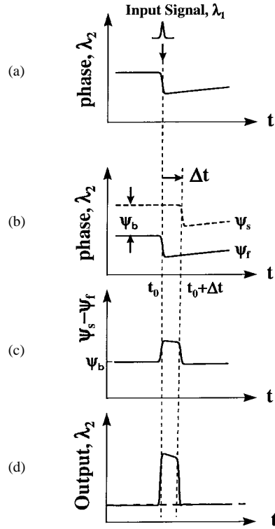
Fig. 2. Wavelength-conversion mechanism. (a) Band-filling-induced transient phase change for the \lambda_2 CW after the SOA. (b) Time delay between phase changes for the two split components after the split-delay. (c) The time-dependent phase components after t_0 + \Delta t are cancelled with each other. (d) Output intensity.
