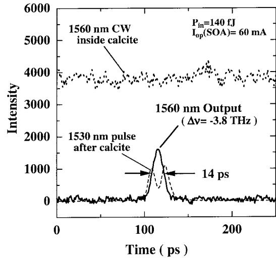
Fig. 3. Streak-camera trace (resolution = 8 ps) for the 1560-nm output (solid line). The output pulsewidth matched the calcite delay time of 14 ps indicated by the dashed line. This pulsewidth was much shorter than the separately measured carrier recovery time of 200 ps in this SOA.
